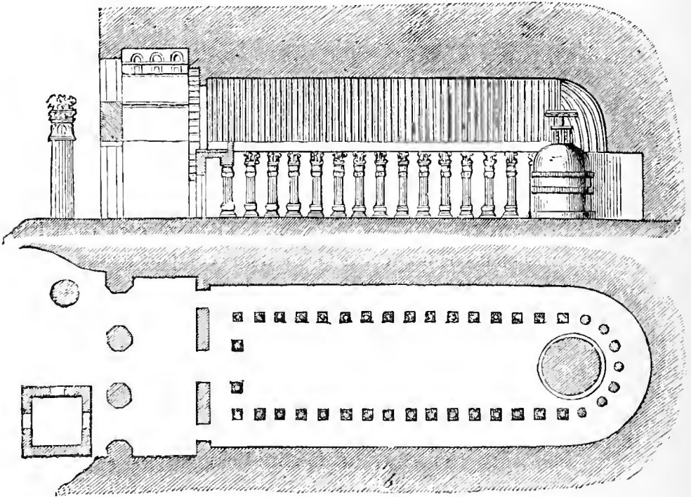
FIG. 40.—CHAITYA NEAR POONA.
